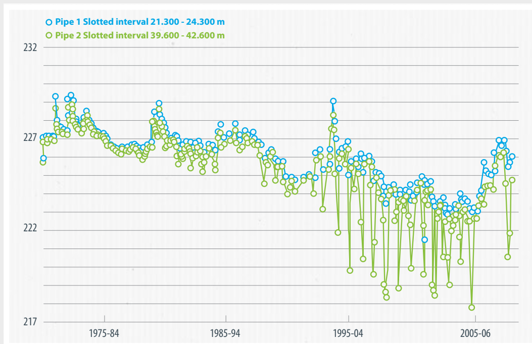
Figure 21 An example hydrograph of groundwater levels in the Namoi Valley
